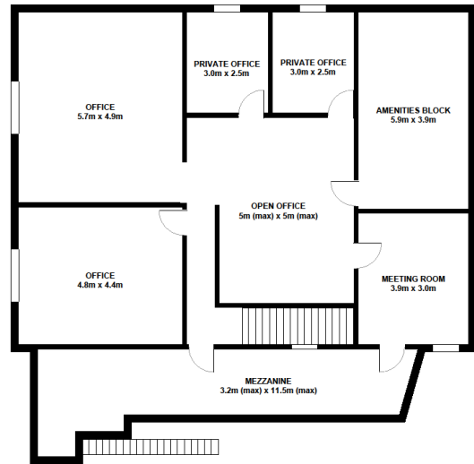
FIRST FLOOR OFFICES
